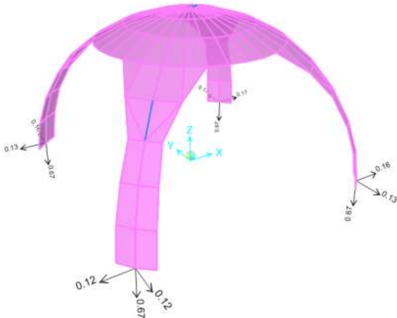
Max Reaction (Uplift) N^* = 0.7 \text{ kN}
