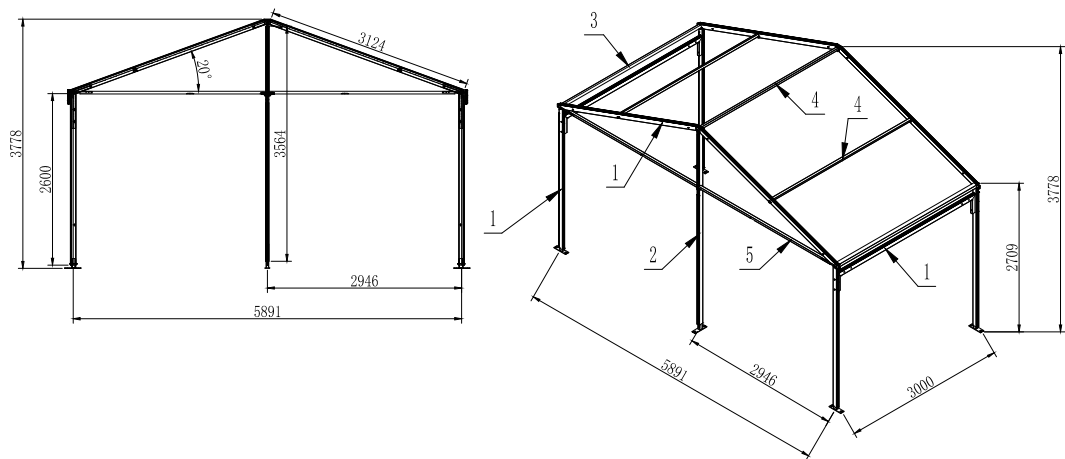
6m Span (3m Bay)
