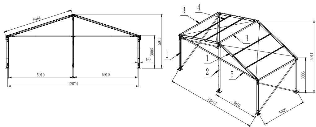
12m Span (5m Bay)
